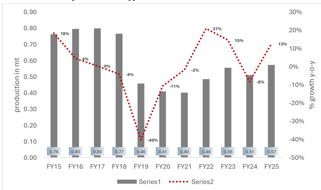
Chart 59: Domestic production of copper
