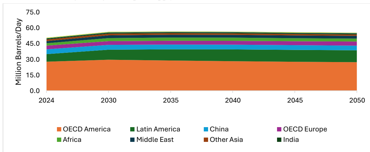
Chart 51: Long Term global liquid supply outlook
