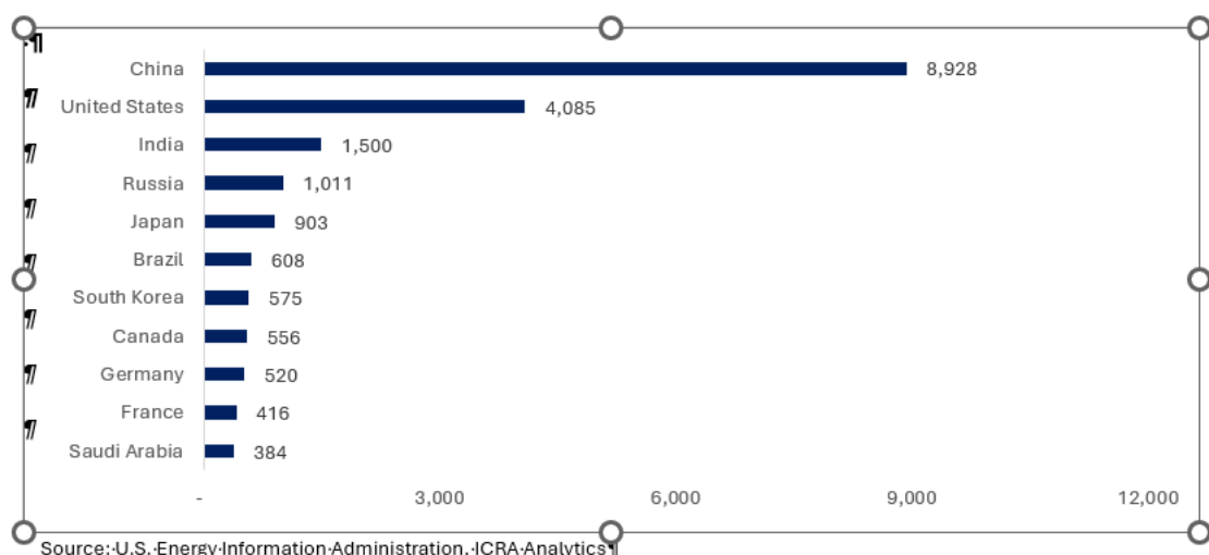
Chart 80: Electricity Net Consumption (billion kWh) for 2023
